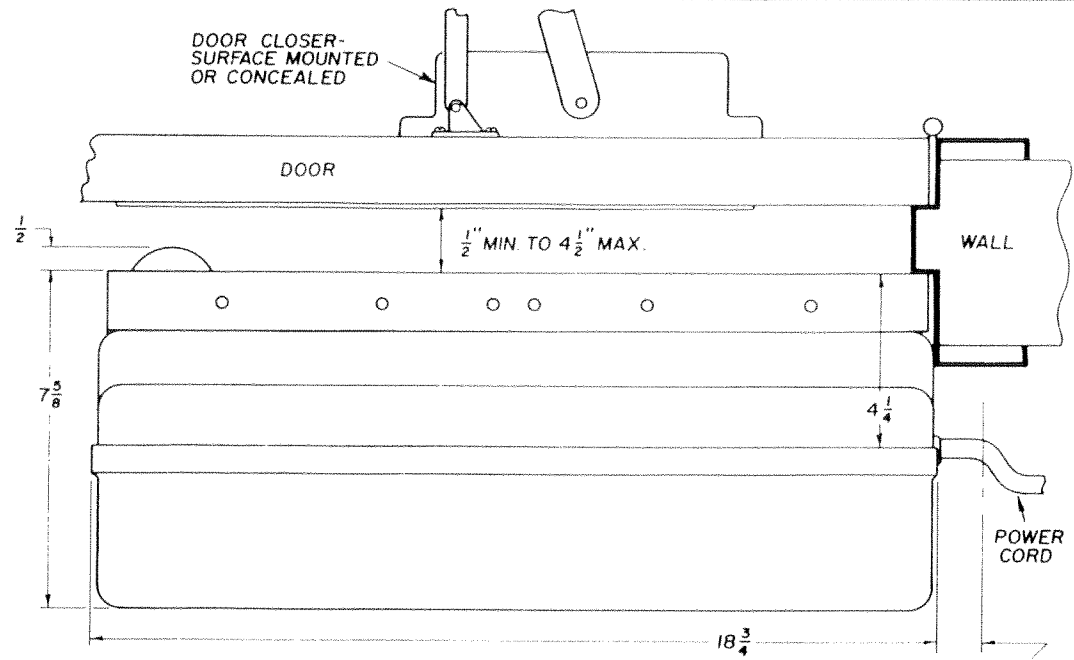
TOP VIEW RIGHT HAND UNIT
