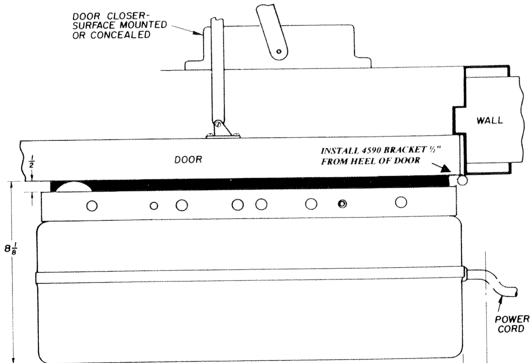
TOP VIEW LEFT HAND UNIT
