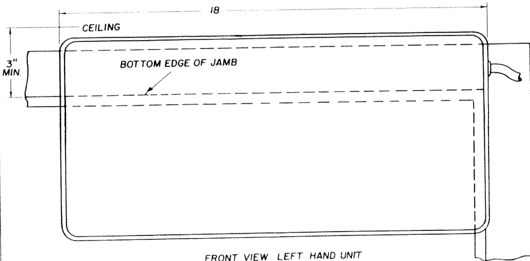
FRONT VIEW LEFT HAND UNIT
