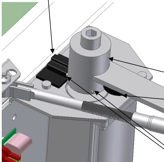
VELCROED SENSOR
